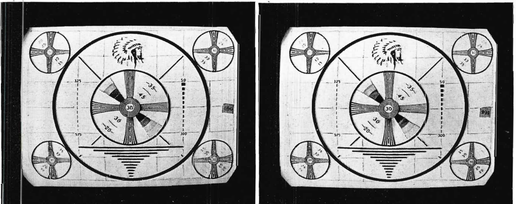
FIG. 3(a). WM-20A Demodulator Monitor presentation of required partially suppressed lower sideband transmission characteristic, as sampled between sideband filter and diplexer. Distortion including leading whites and trailing smears inherent to suppression of the lower sideband is in evidence. A slight amount of ringing evident at 350 lines, resulting from necessary 20 db r-f sound carrier trap in demodulator.
