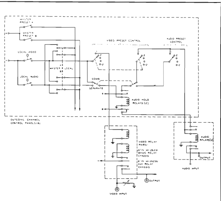
FIG. 12. Simplified diagram—Preset Audio/Video Master Control Switching used at KECA, Los Angeles, Calif.
