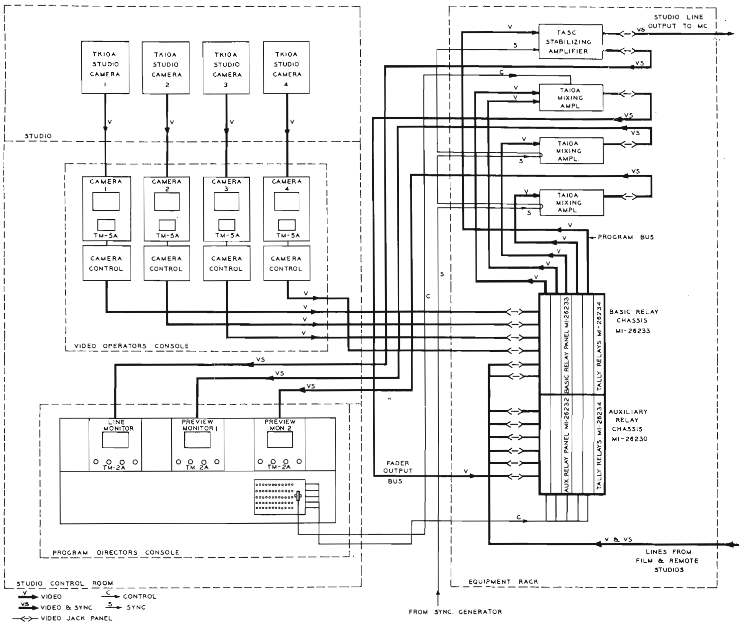
FIG. 7. Block diagram showing how the video facilities may be extended by adding the Program Console with Program Bus Output.
