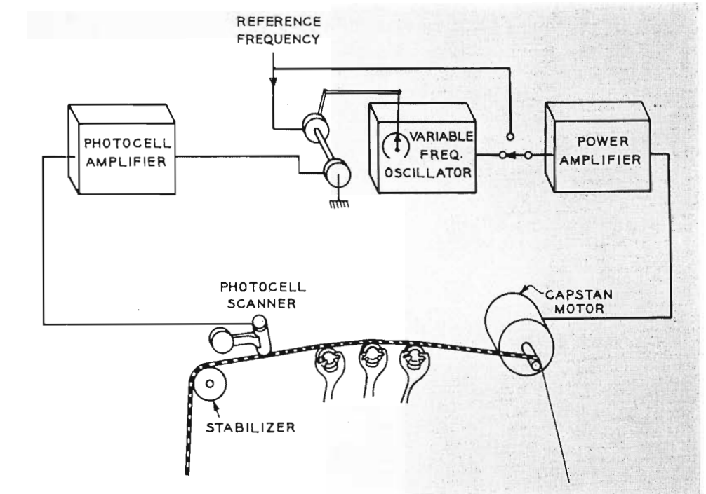
FIG. 3. Block diagram illustrating the operation of complete system.
