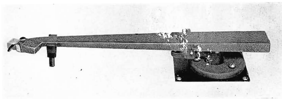
FIG. 16 (above. View of the final design of the Lightweight Tone Arm complete with Pickup, mounting plate and arm rest.
