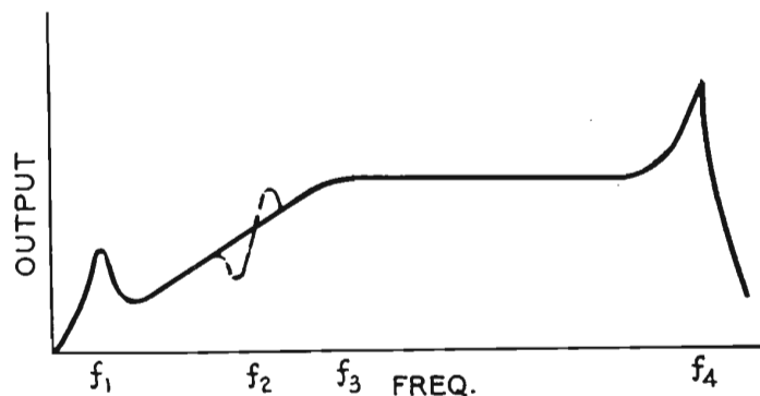
TYPICAL RESPONSE (a)
