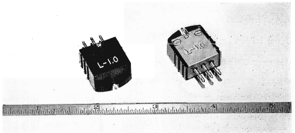
FIG. 4 (below). Size: approximately ¾" x ⅜" x ¼". Weight: approximately ½ ounce.
