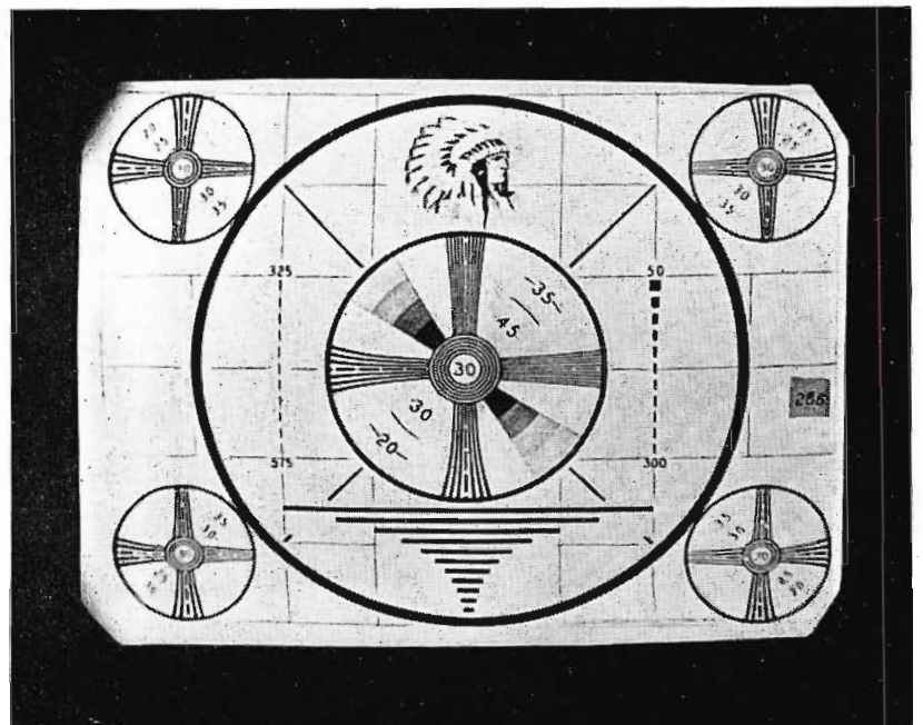
FIG. 2(a). Diode detection of essentially double sideband transmitter output, indicating smearing at approximately 400 lines (over 5 mc) on vertical wedge—a result of 5 mc video cutoff characteristic of this location. FIG. 2(b). ▼
