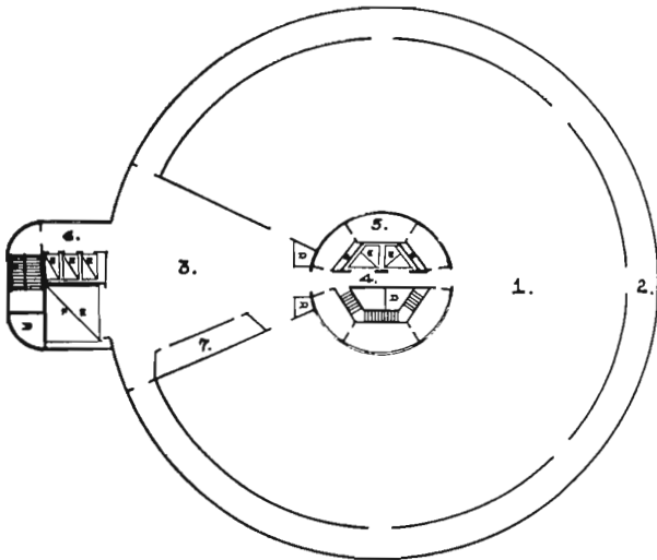
TYPICAL T.V. STUDIO FLOOR PLAN.
