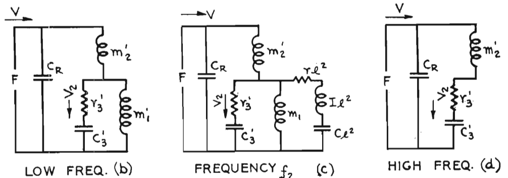
FIG. 5 (at right). Typical Response Curve of the combination and equivalent low-, medium- and high-frequency circuits of Pickup and Tone Arm.
