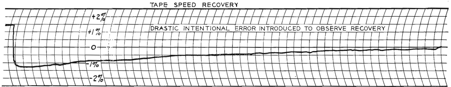
FIG. 7. Curve showing the speed of recovery after intentional error has been introduced.
