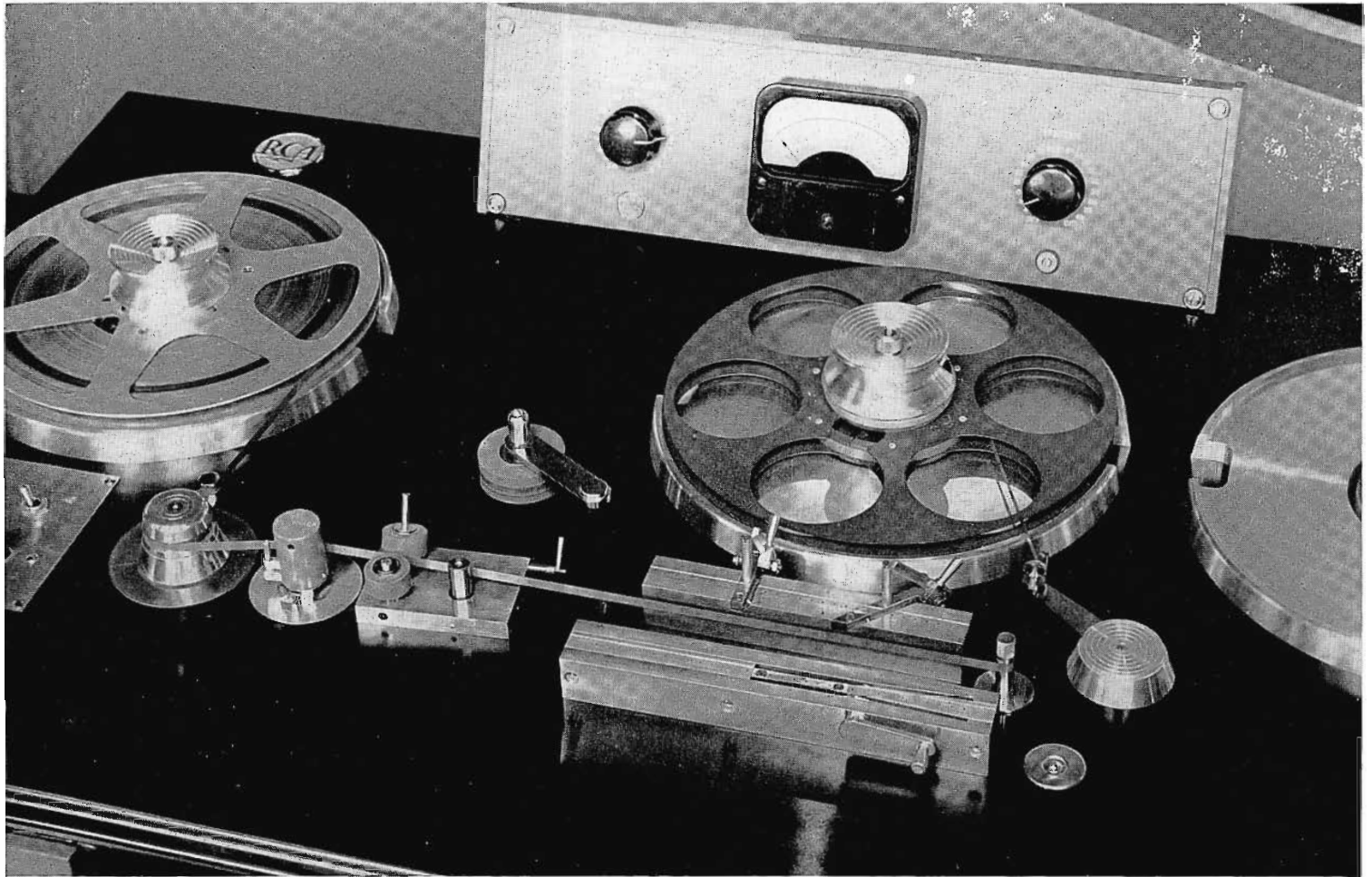
FIG. 1. Closeup view of the Magnetic Tape Editing Machine. Editing Accessories, and machine components are shown left to right: Control Panel, Stabilizer, Reproducing Head, Tape Marker, Capstan Tape Cutting and Splicing Bars, Vacuum System Switch and one of reel drive tape take-up arms.
