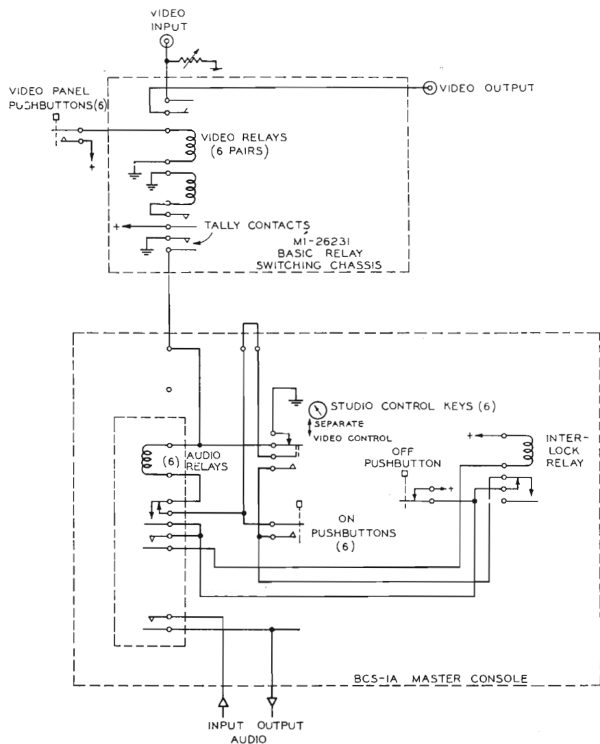
FIG. 10. Simplified schematic diagram showing control circuits for Audio/Video Master Control Switching. (Note in diagram that one relay or pair of contacts may actually be two or more in an interlocking circuit or in several identical circuits.)
