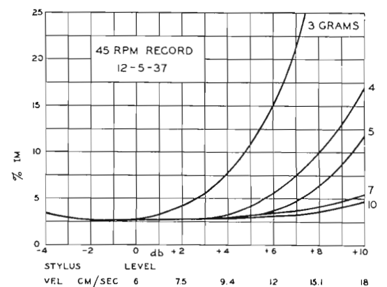
FIG. 5. Characteristics obtained with MI-11874 pickup when using the 45 rpm test record.
