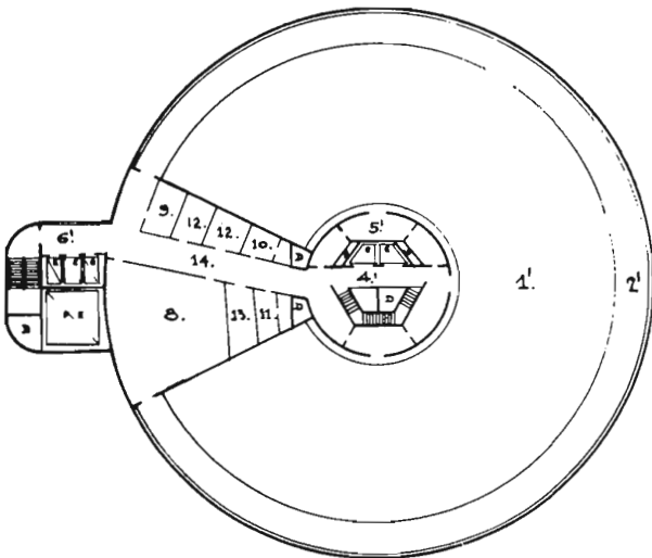
TYPICAL T.V. INTERMEDIATE LEVEL STUDIO FL. PL.
